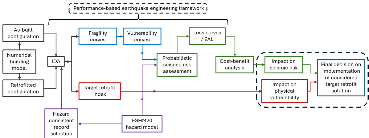
Figure 1- Flowchart of the proposed framework for quantifying the impact of target retrofit solutions on reduction of seismic risk
