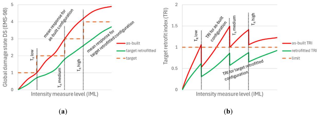
Figure 2- (a) Conceptual performance curves for the as-built and retrofitted configurations. The orange line represents the target behaviour for the building; (b) Target retrofit index (TRI) for the as-built and retrofitted configurations, with the TRI=1 orange line indicating the threshold of acceptable performance (TRI<1) or limit exceeded (TRI>1)
