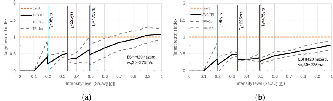
Figure 6- Target retrofit index (TRI) within one standard deviation for the (a) as-built and (b) retrofitted configuration. Dashed orange lines represents the TRI=1 threshold
