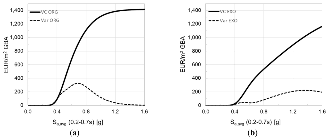
Figure 8- New vulnerability curves and their variances for the (a) as-built and (b) retrofitted configuration
