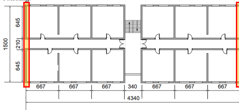
Figure 3- Characteristic floor layout of the selected case study building with marked locations of the target retrofit solution
