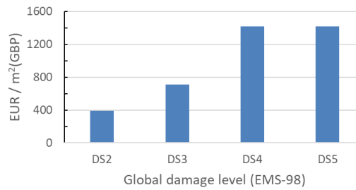
Figure 7- Deterministic damage-to-loss model adopted for this study, simulating to an extent the post-earthquake reconstruction praxis in Croatia after the 2020 earthquakes
