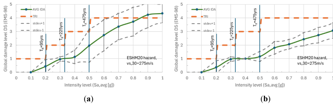
Figure 5- Mean IDA results and one standard deviation for the (a) as-built and (b) retrofitted configuration. Dashed orange lines represent the target behaviour according to Table 1
