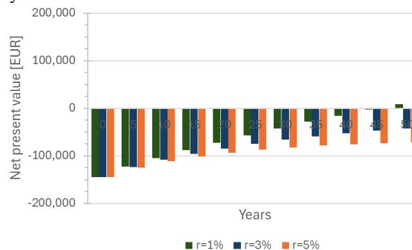
Figure 10- Net present values for the proposed remaining building lifespan of 50 years for three discount rates r
