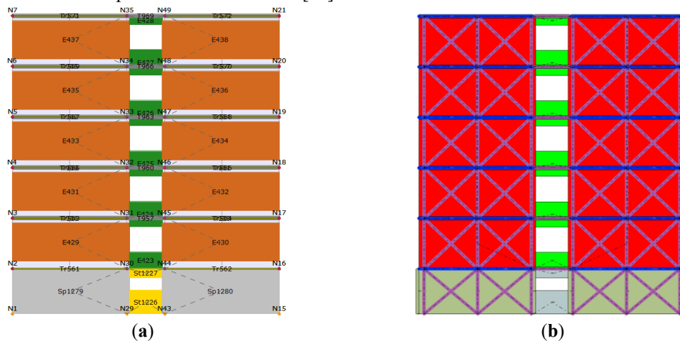
Figure 4- Outer façade wall in the critical transversal direction for (a) as-built and (b) retrofitted configuration
